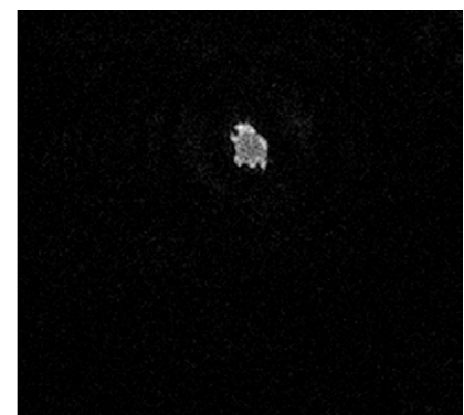
Reconstruction of the particle image from the hologram above. The length scale is not calibrated here, but the particle is likely 50-100 microns in size.
